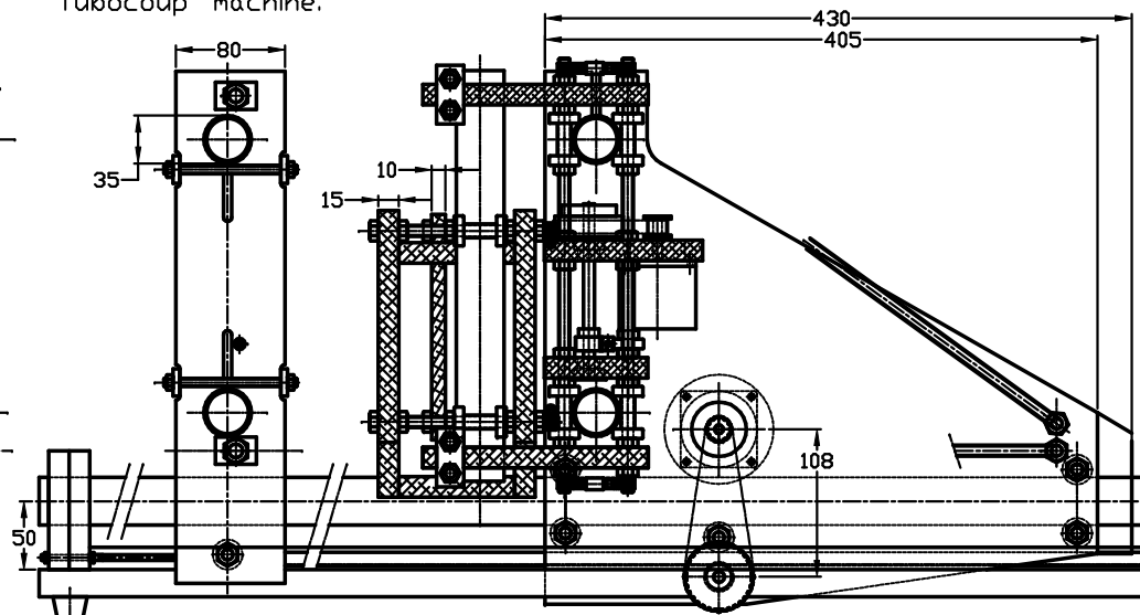
(c) Pierre ROUZEAU 2005. 'Tubocoup' machine.
