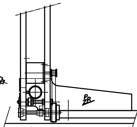
(c) Pierre ROUZEAU 2005. 'Tubocoup' machine.
