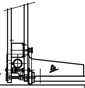
(c) Pierre ROUZEAU 2005. 'Tubocoup' machine.
