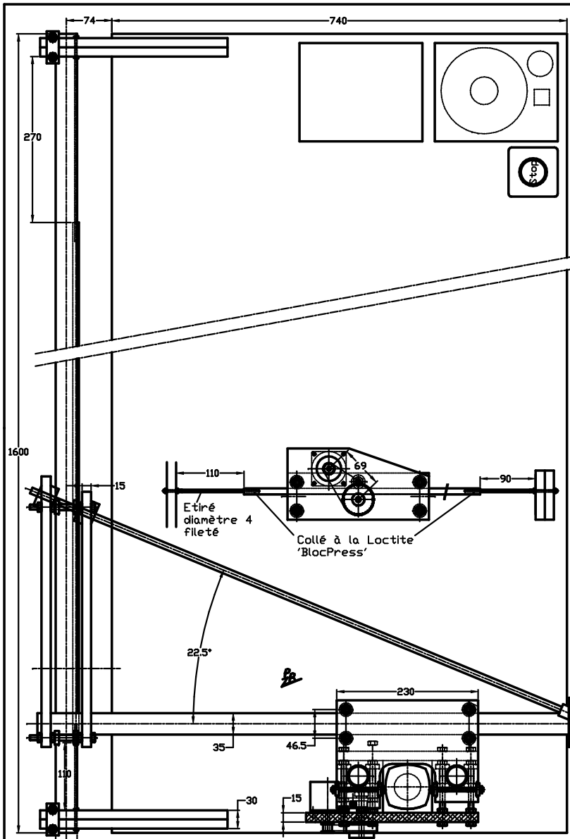
(c) Pierre ROUZEAU 2005. 'Tubocoup' machine.
